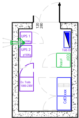
Amenagement armoires
