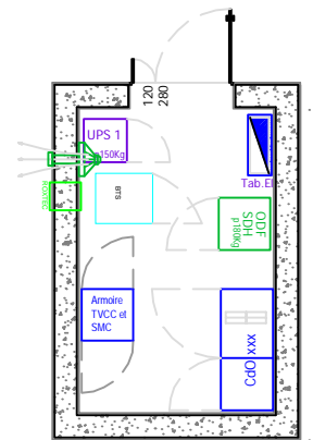
Amenagement armoires
