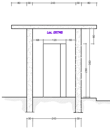
Plan elevation
