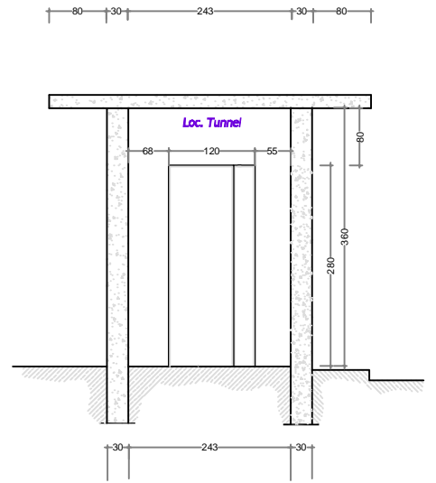
Plan elevation
